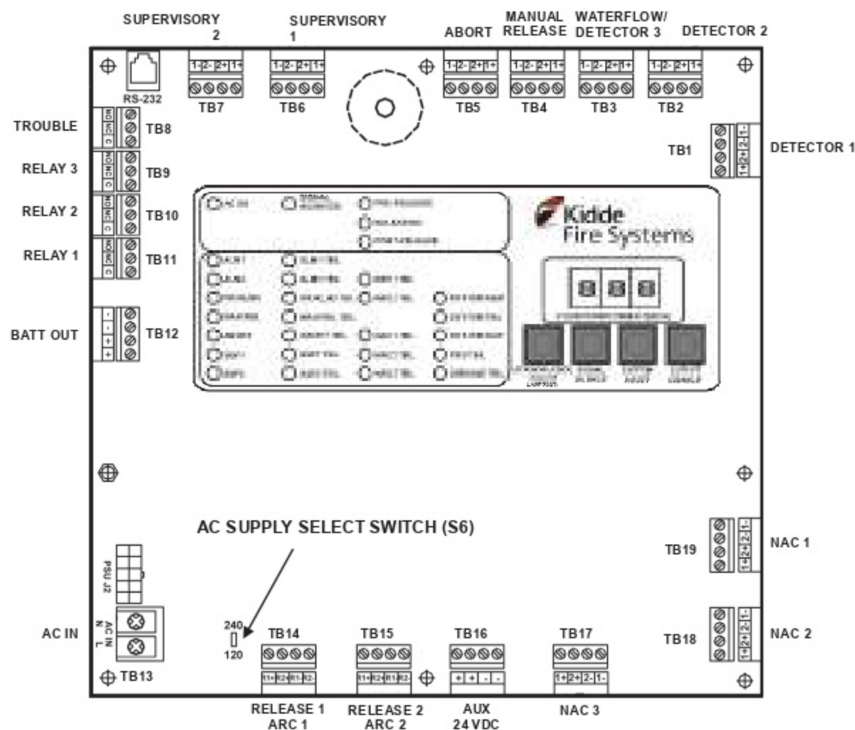
Figure 1. Printed Circuit Board (PCB)
